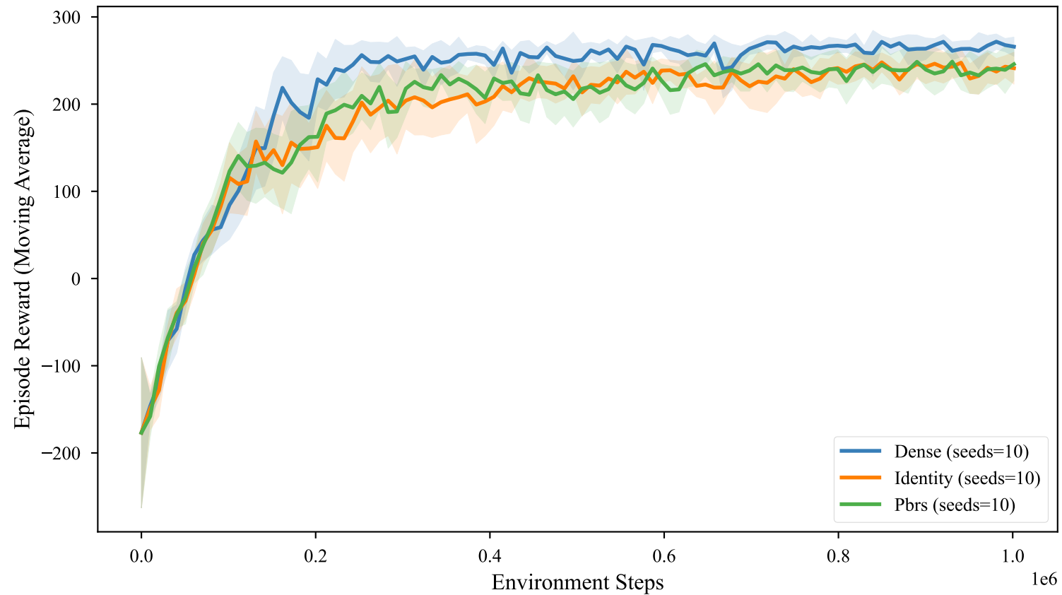
PPO Training Performance on LunarLander-v3 (True Unshaped Objective)
