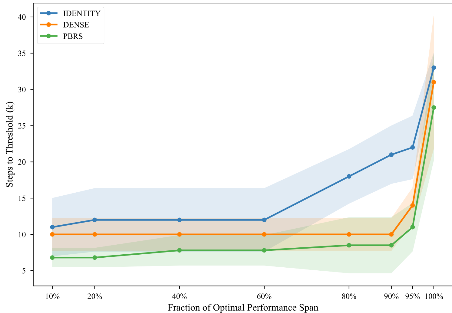
Sample Efficiency Curve on Acrobot-v1
