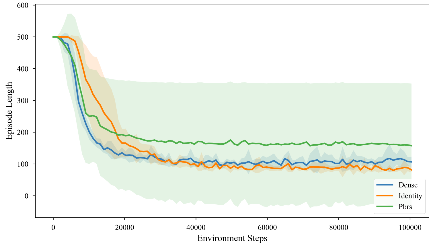
PPO Episode Lengths during Training on Acrobot-v1
