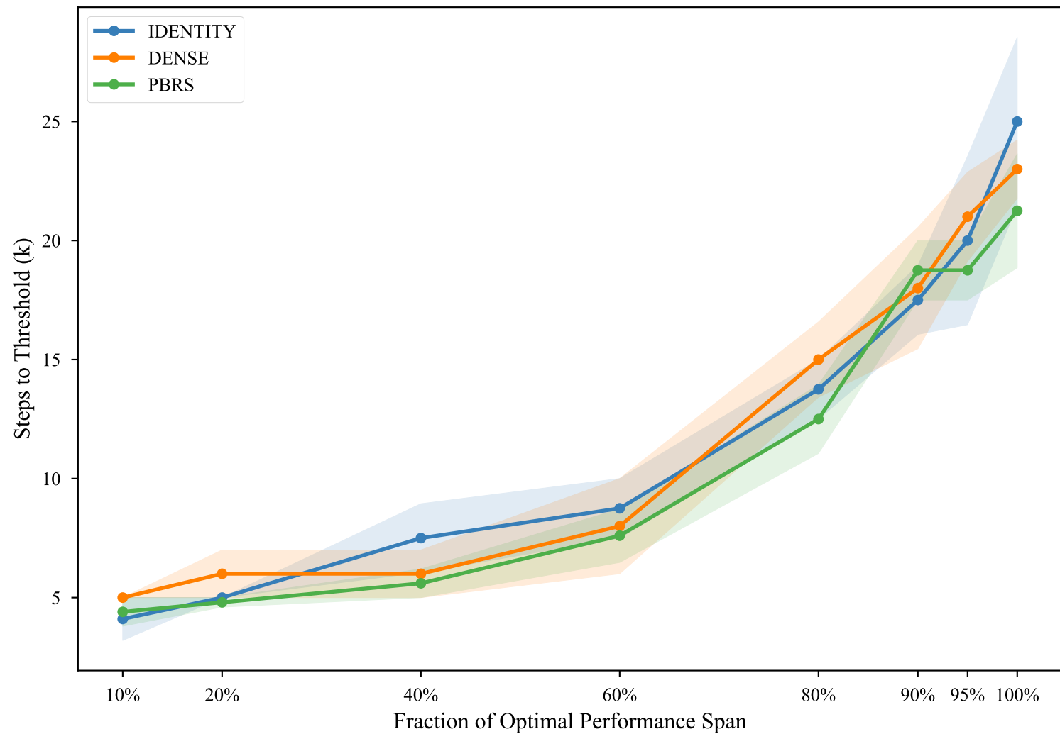
Sample Efficiency Curve on CartPole-v1
