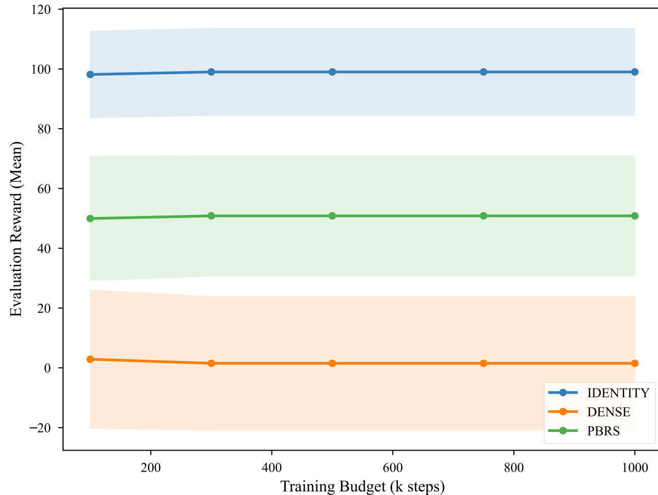
Asymptotic Performance vs. Training Budget Limit
