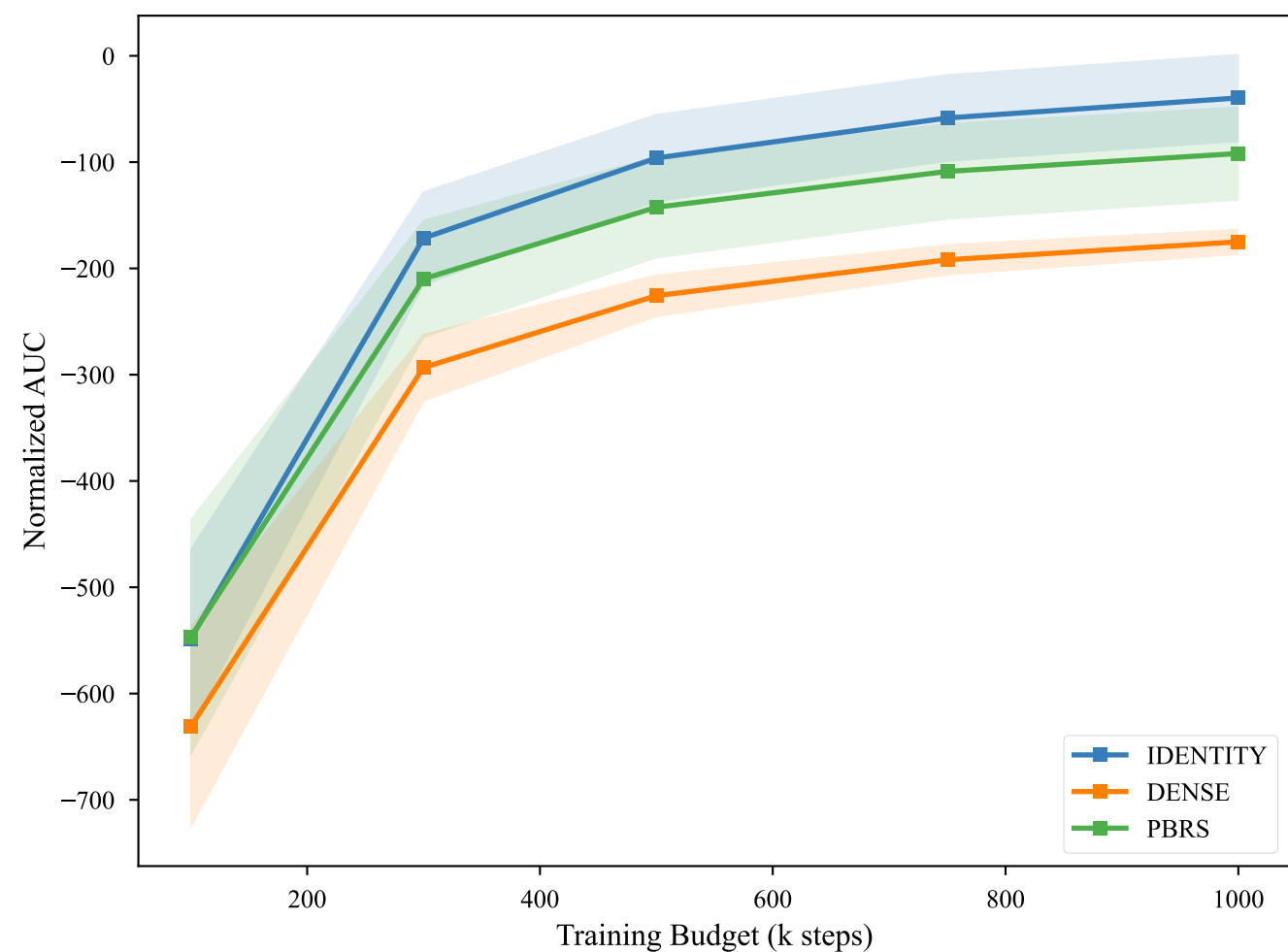
Sample Efficiency (AUC) vs. Training Budget Limit
