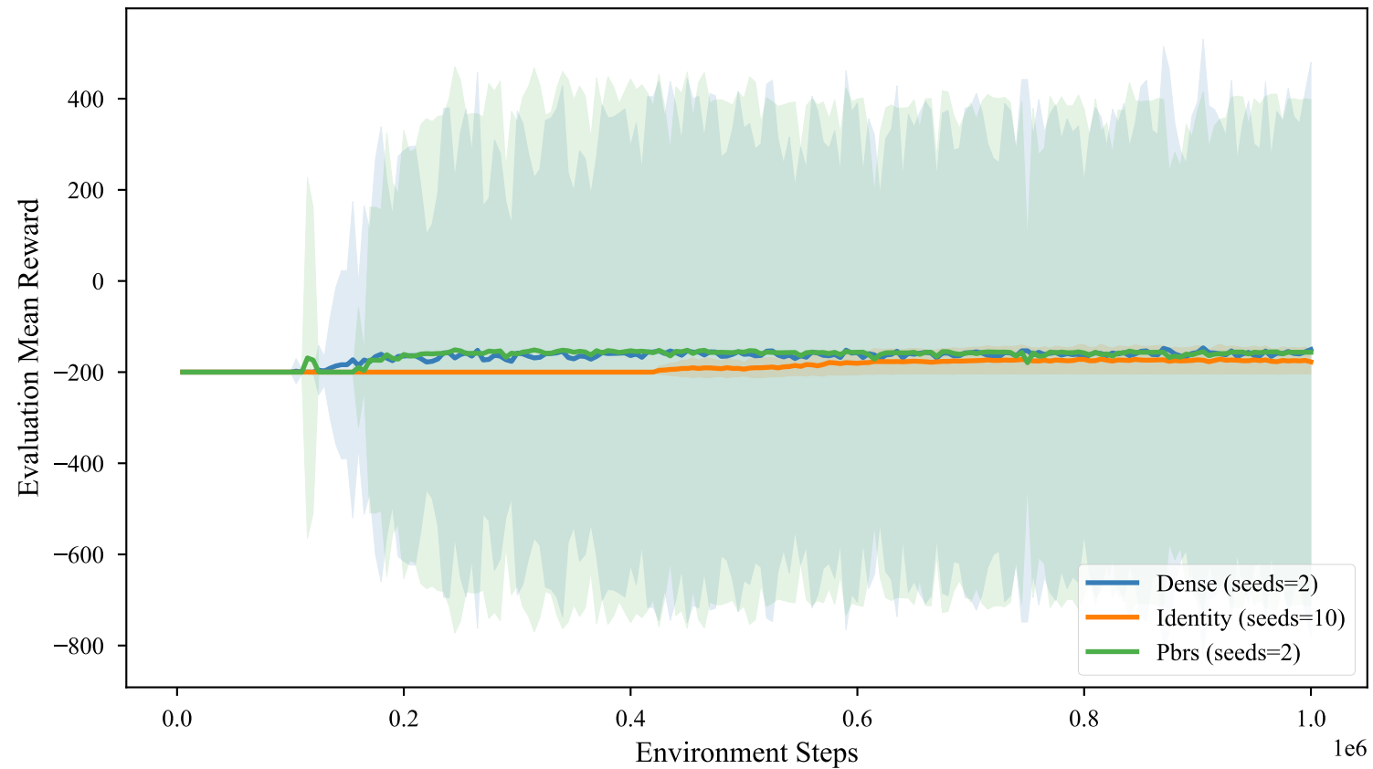
PPO Evaluation Performance on MountainCar-v0 (Deterministic, Unshaped)
