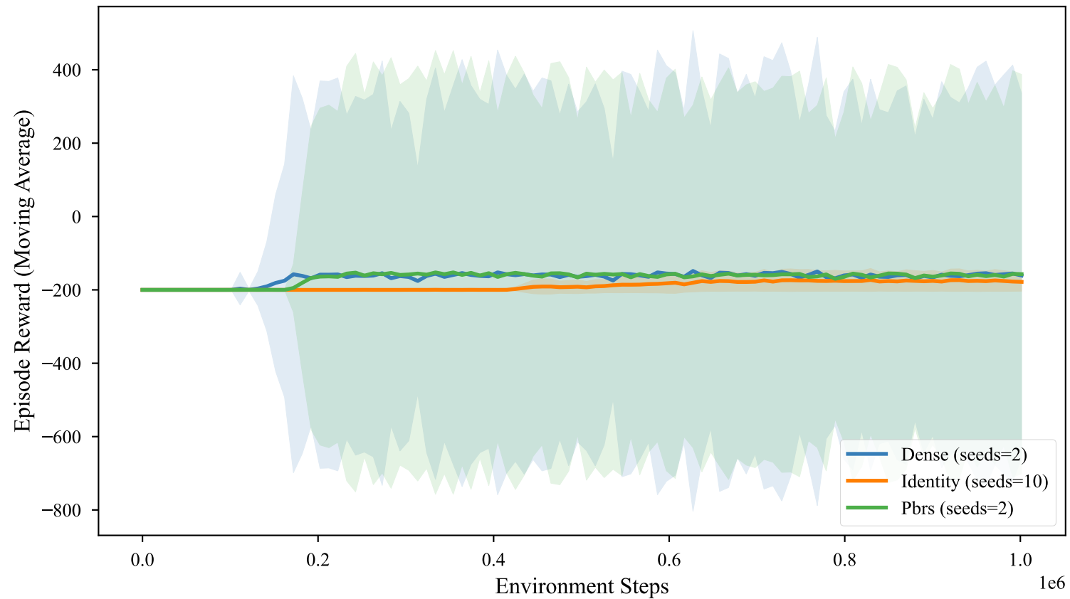
PPO Training Performance on MountainCar-v0 (True Unshaped Objective)
