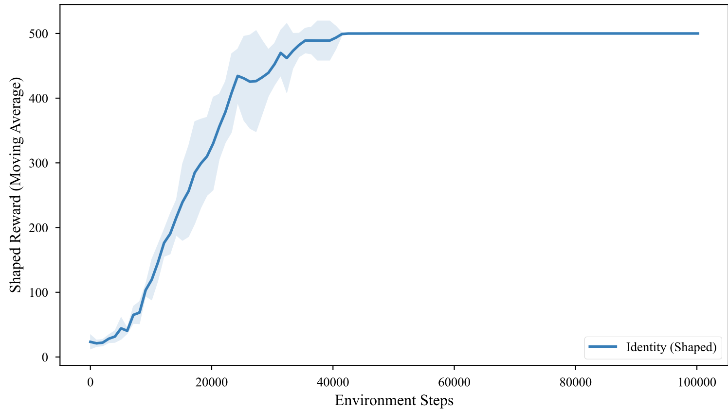
PPO Training Performance on CartPole-v1 (Proxy Shaped Objective)
