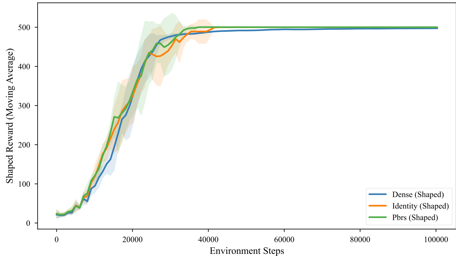
PPO Training Performance on CartPole-v1 (Proxy Shaped Objective)
