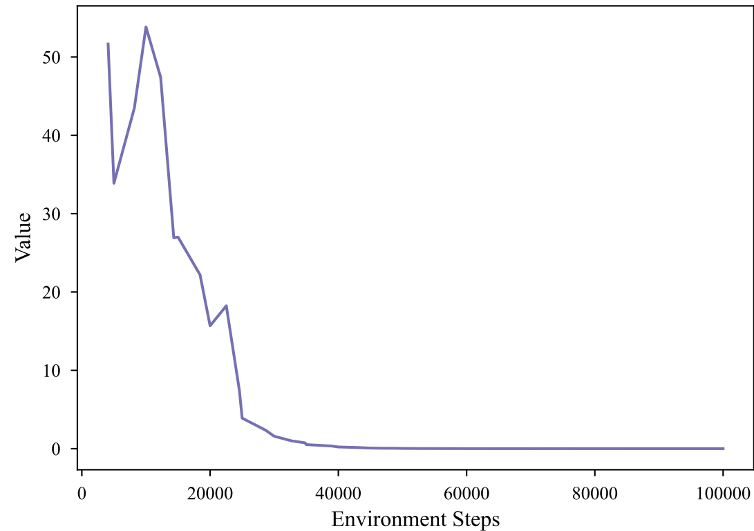
Policy Entropy Loss
