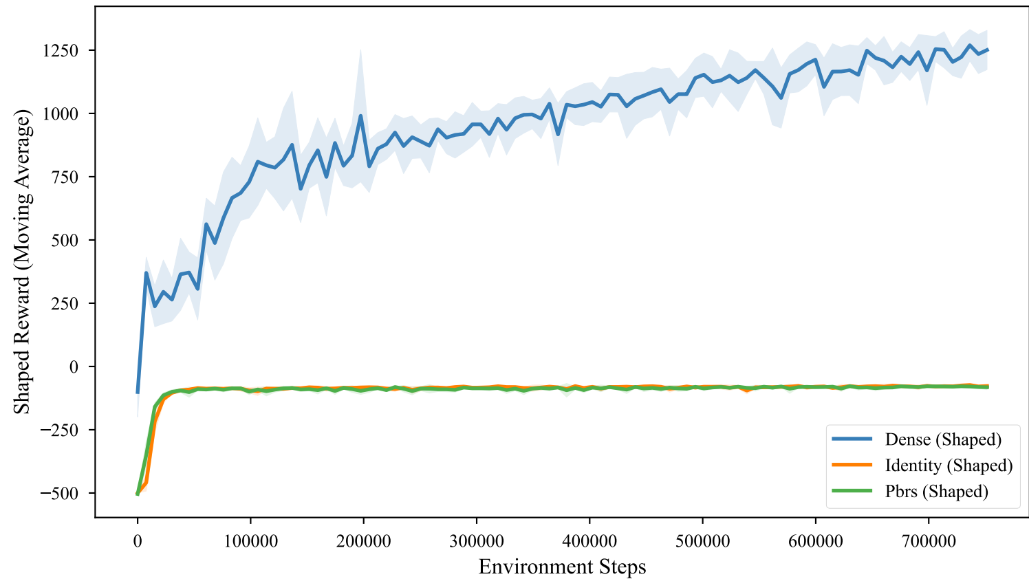
PPO Training Performance on Acrobot-v1 (Proxy Shaped Objective)
