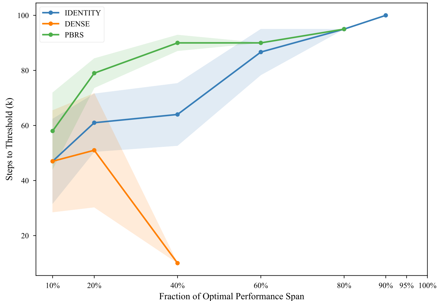
Sample Efficiency Curve on LunarLander-v3
