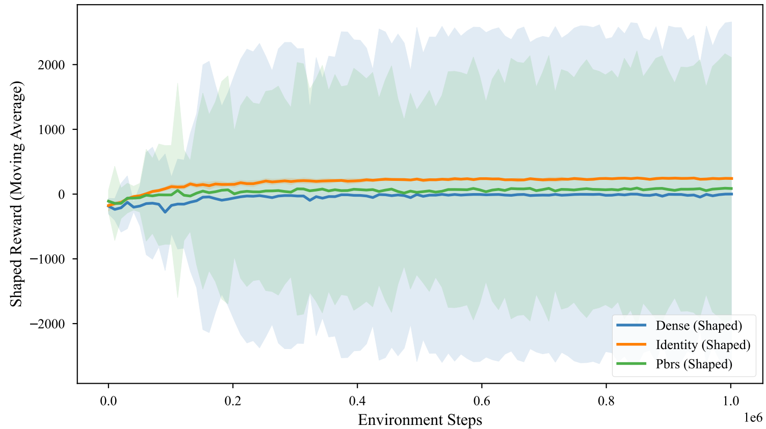
PPO Training Performance on LunarLander-v3 (Proxy Shaped Objective)
