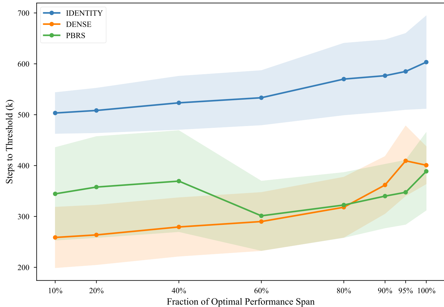
Sample Efficiency Curve on MountainCar-v0
