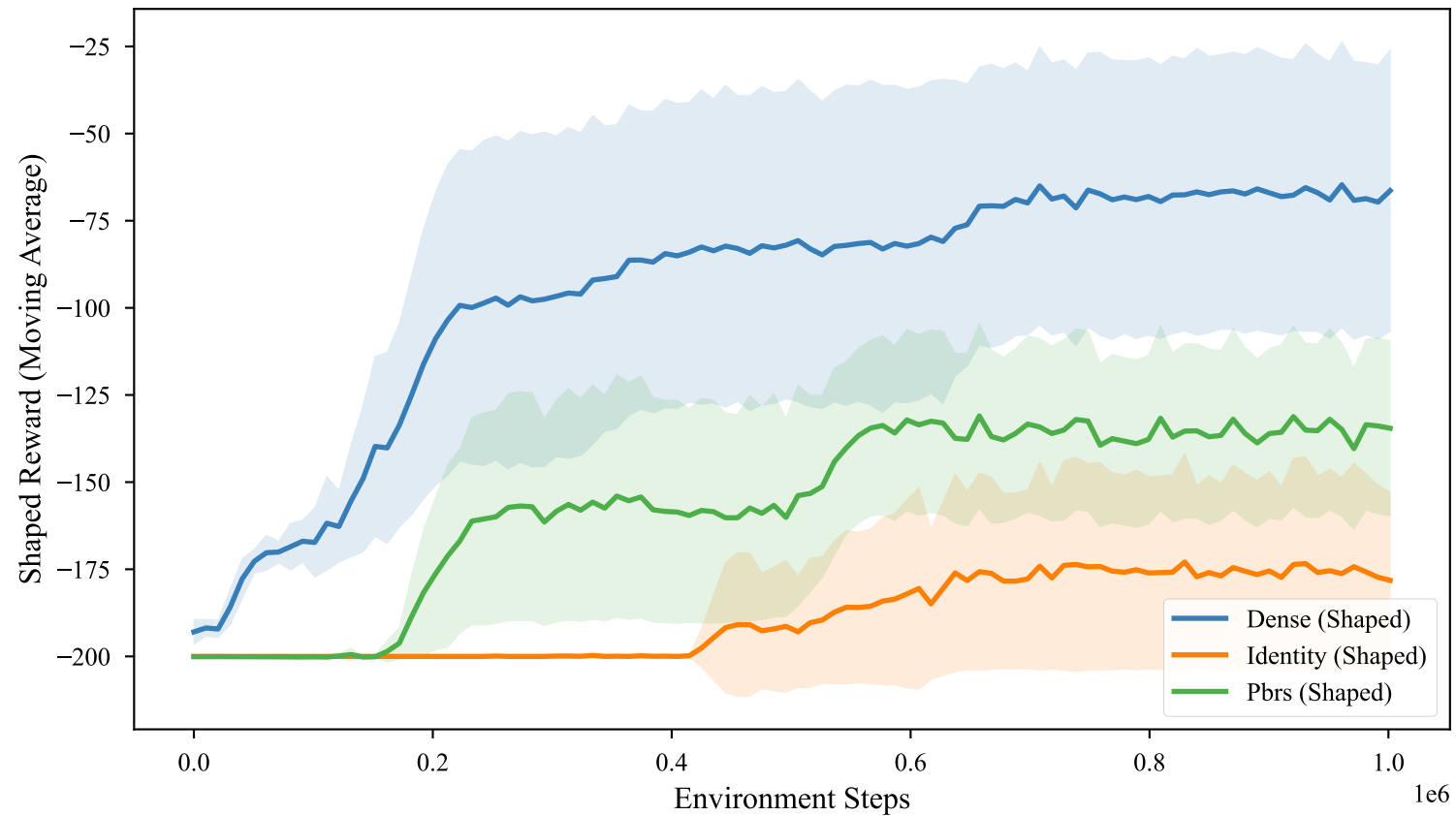
PPO Training Performance on MountainCar-v0 (Proxy Shaped Objective)
