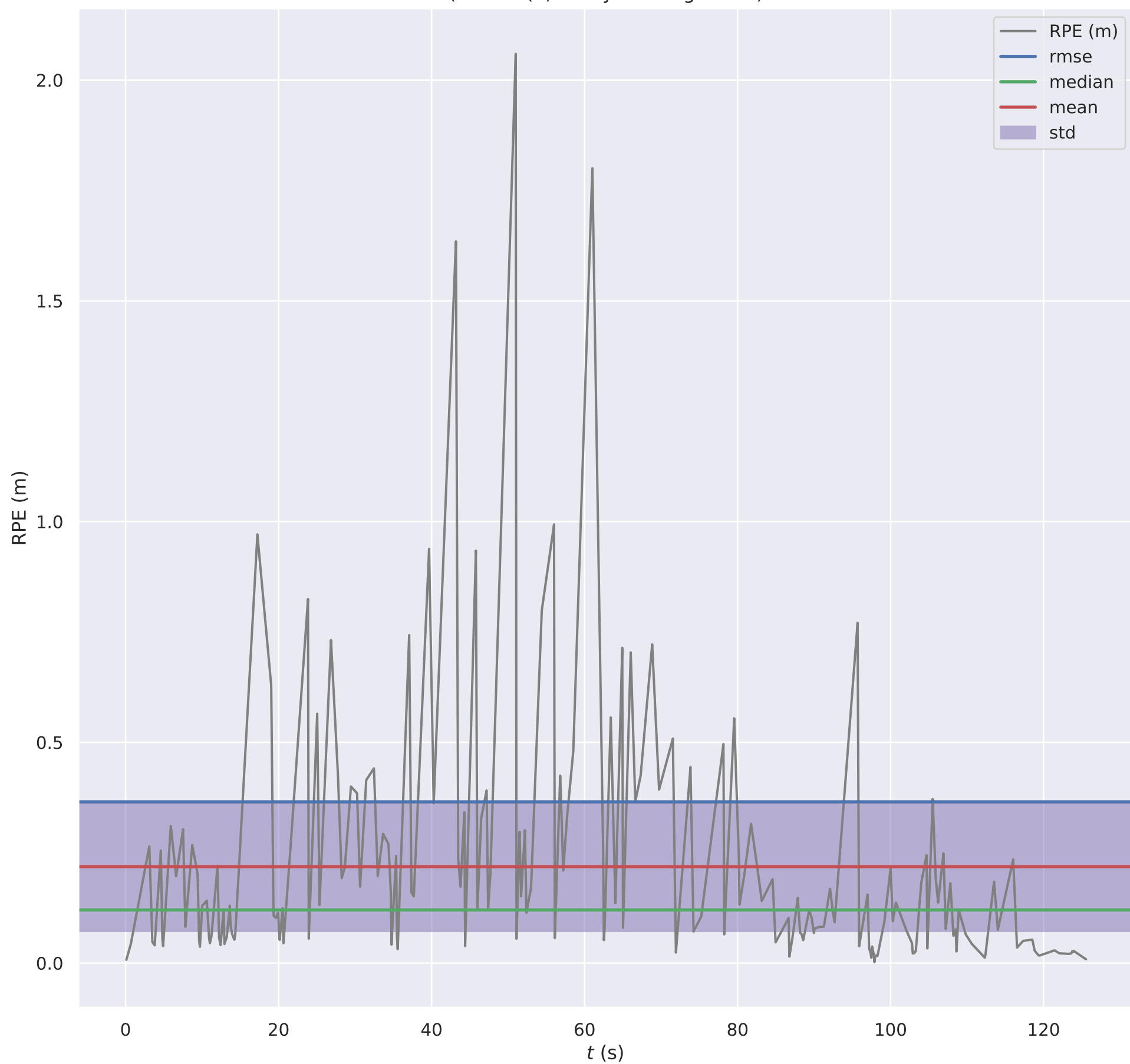
RPE w.r.t. translation part (m) for \delta = 1 (frames) using consecutive pairs (with SE(3) Umeyama alignment)
