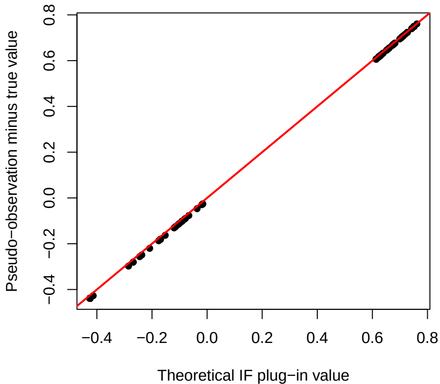
F( \tau ), setting 1, n=200
