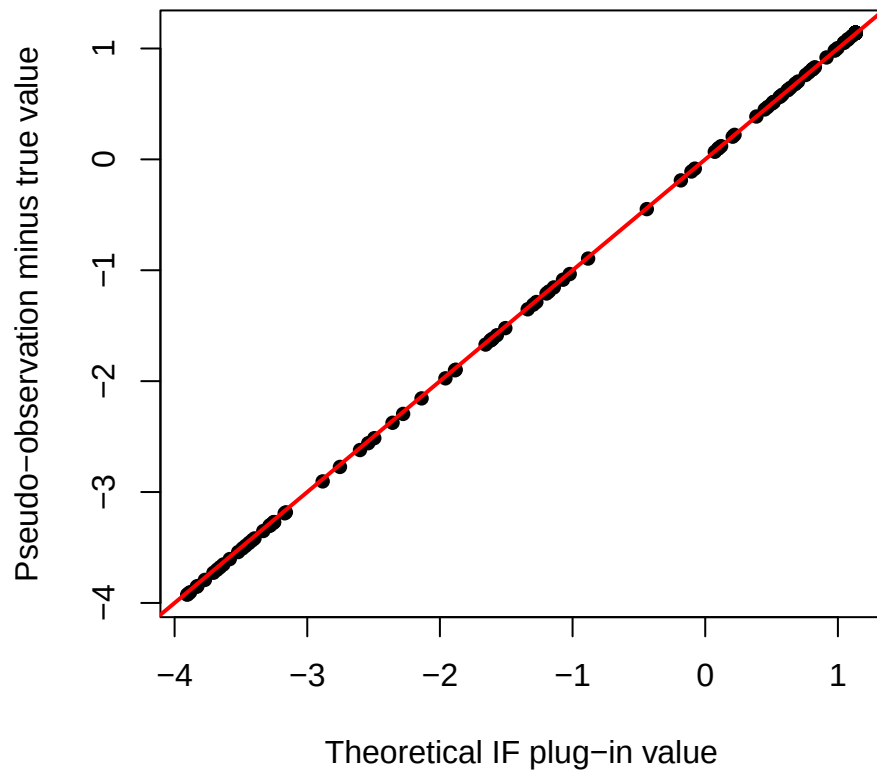
RMST, setting 1, n=200
