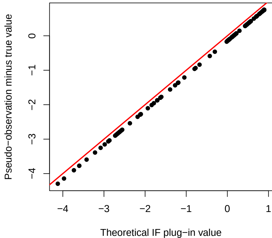
RMST, setting 2, n=200
