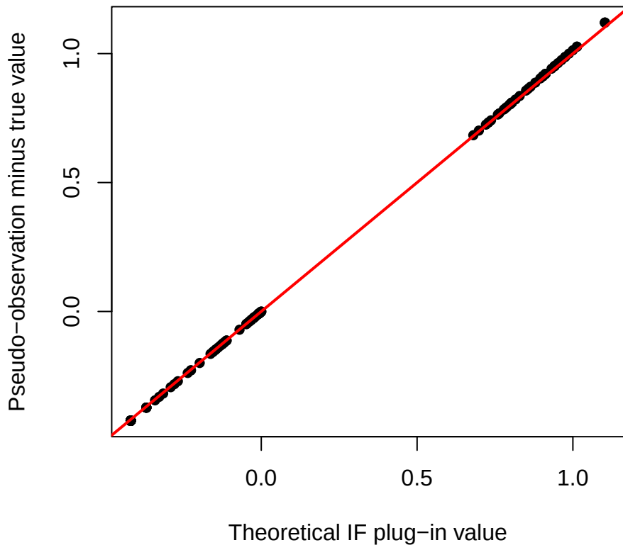
F( \tau ), setting 2, n=200
