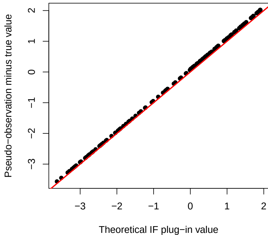
RMST, setting 3, n=200
