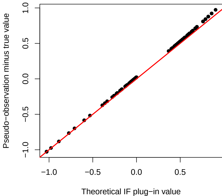
F( \tau ), setting 3, n=200
