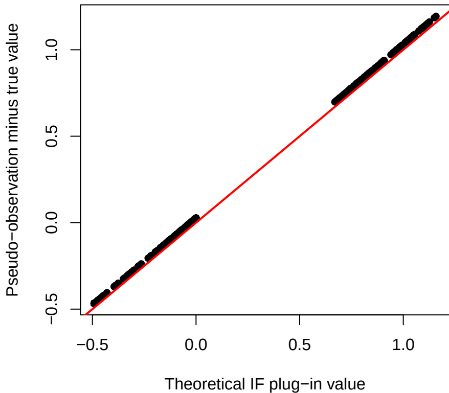
F( \tau ), setting 2, n=500
