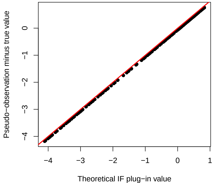
RMST, setting 2, n=500
