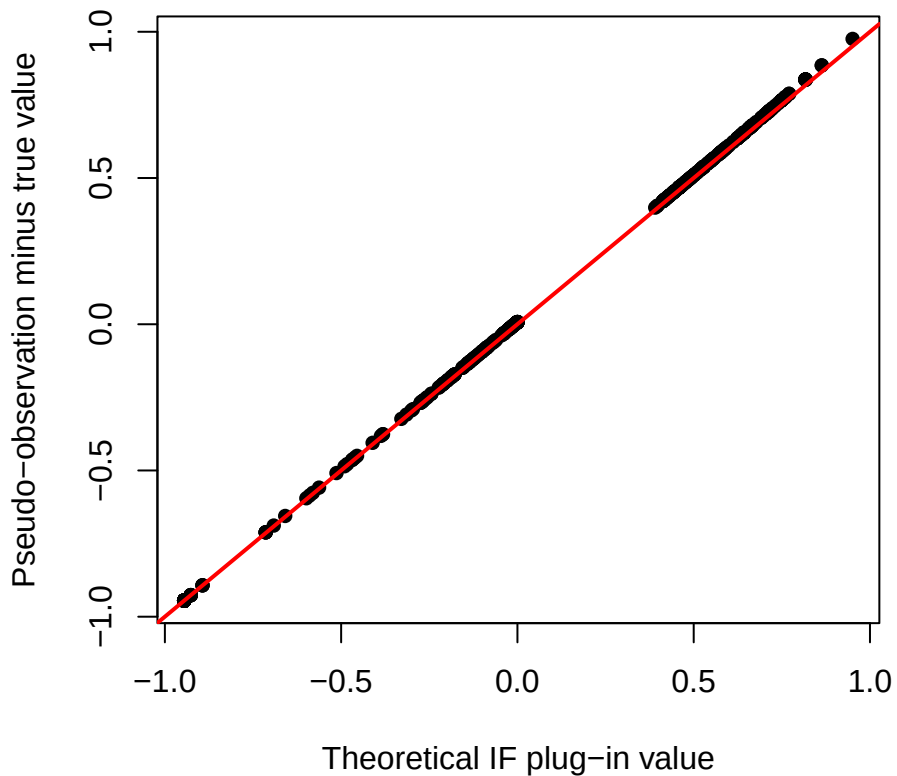
F( \tau ), setting 3, n=500
