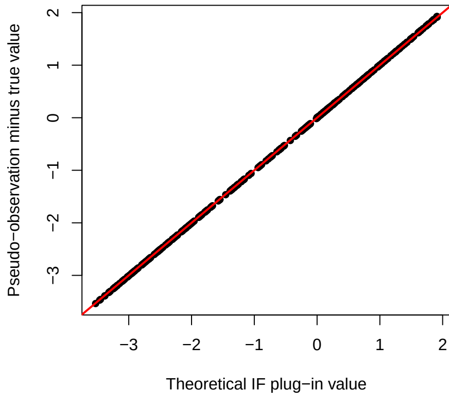
RMST, setting 3, n=500
