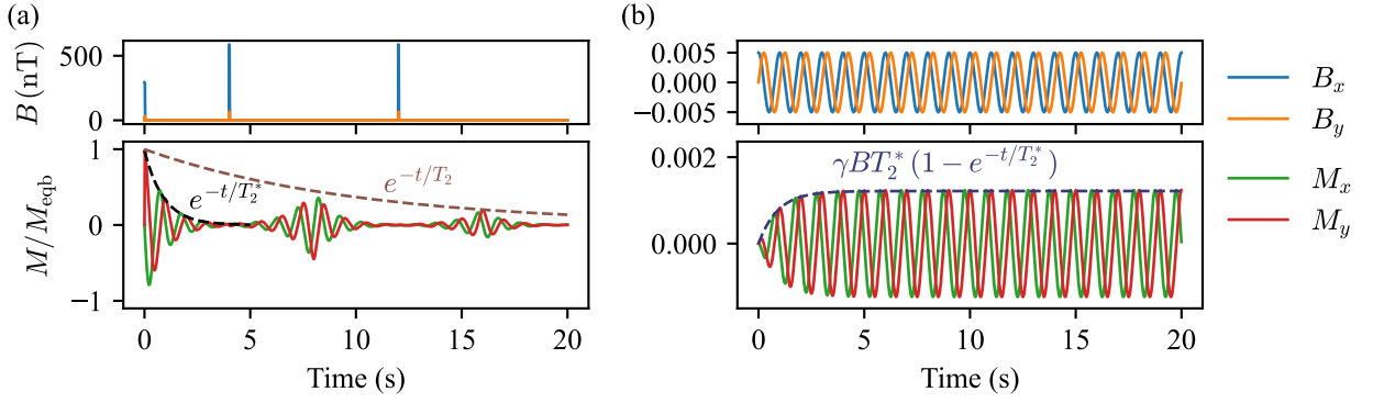
FIG. 3. Simulated magnetic fields in x and y directions (upper row) and induced NMR signals (lower row). The magnetizations plotted are normalized by equilibrium magnetization. (a) After 90^\circ and 180^\circ magnetic-field pulses in x-y plane, free decay (relaxation time T_2^* ) and echo signals (relaxation time T_2 ) are generated. (b) Excited by a weak CW magnetic field, the NMR signals increase with \gamma B T_2^* (1 - e^{-t/T_2^*}) , where B = \sqrt{B_x^2 + B_y^2} is the magnitude of the excitation. Hendrik: In (a)-top, why is there a nonzero B_y component at the pulses? Yuzhe: This indicates the orientation of the magnetic pulse. The pulse is like aB_x + bB_y .
