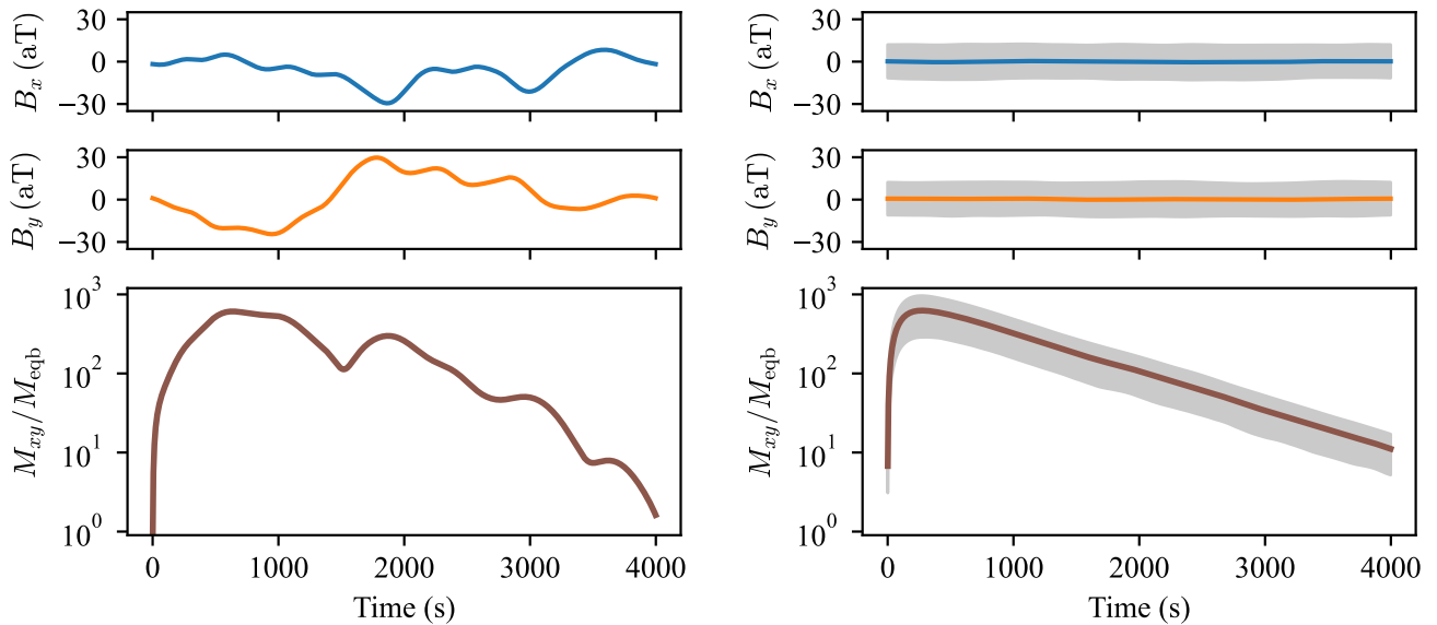
FIG. 6. Simulations of local virialized axion dark matter halo. From top to bottom: pseudomagnetic fields in the transverse plane ( B_x and B_y ) and the transverse magnetization induced ( M_{xy} ). Left: one single simulation. Right: 1000 simulations to account for the stochasticity. The solid lines indicate the value (left column) or mean value (right column) of B_x , B_y , and M_{xy} , while the gray shadows indicate \pm\sigma (standard deviation) range. The sample for the simulations is assumed to be polarized to 50 % initially.
