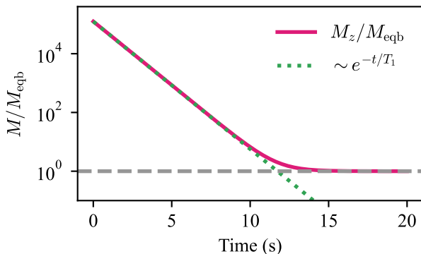
FIG. 4. Simulated T_1 relaxation of a hyperpolarized sample in a static bias field. The axial magnetization M_z is normalized by the equilibrium magnetization M_0 .
