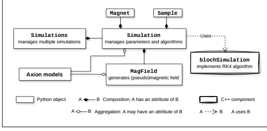
FIG. 2. Architecture of axionbloch . Each Simulation instance imports parameters from Magnet , Sample , and MagField instances. For axion simulations, axion-model objects are required both for Simulation to configure the simulation and for MagField to generate the pseudomagnetic field. Simulations manages one or multiple Simulation instances. Numerical integration is performed via the blochSimulation API, which provides Python access to the underlying C++ implementation.
