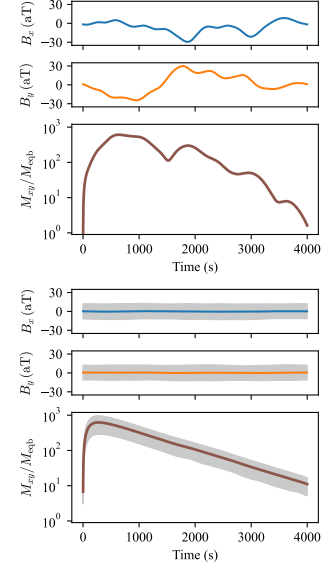
FIG. 6. Simulations of local virialized axion dark matter halo. From top to bottom: pseudomagnetic fields in the transverse plane ( B_x and B_y ) and the transverse magnetization normalized by the equilibrium magnetization ( M_{xy}/M_{eqb} ). Left: one single simulation. Right: 1000 simulations to account for the stochasticity. The solid lines indicate the value (left column) or mean value (right column) of B_x , B_y , and M_{xy} , while the gray shadows indicate the \pm\sigma (standard deviation) range. The sample for the simulations is assumed to be polarized to 50 % initially.
