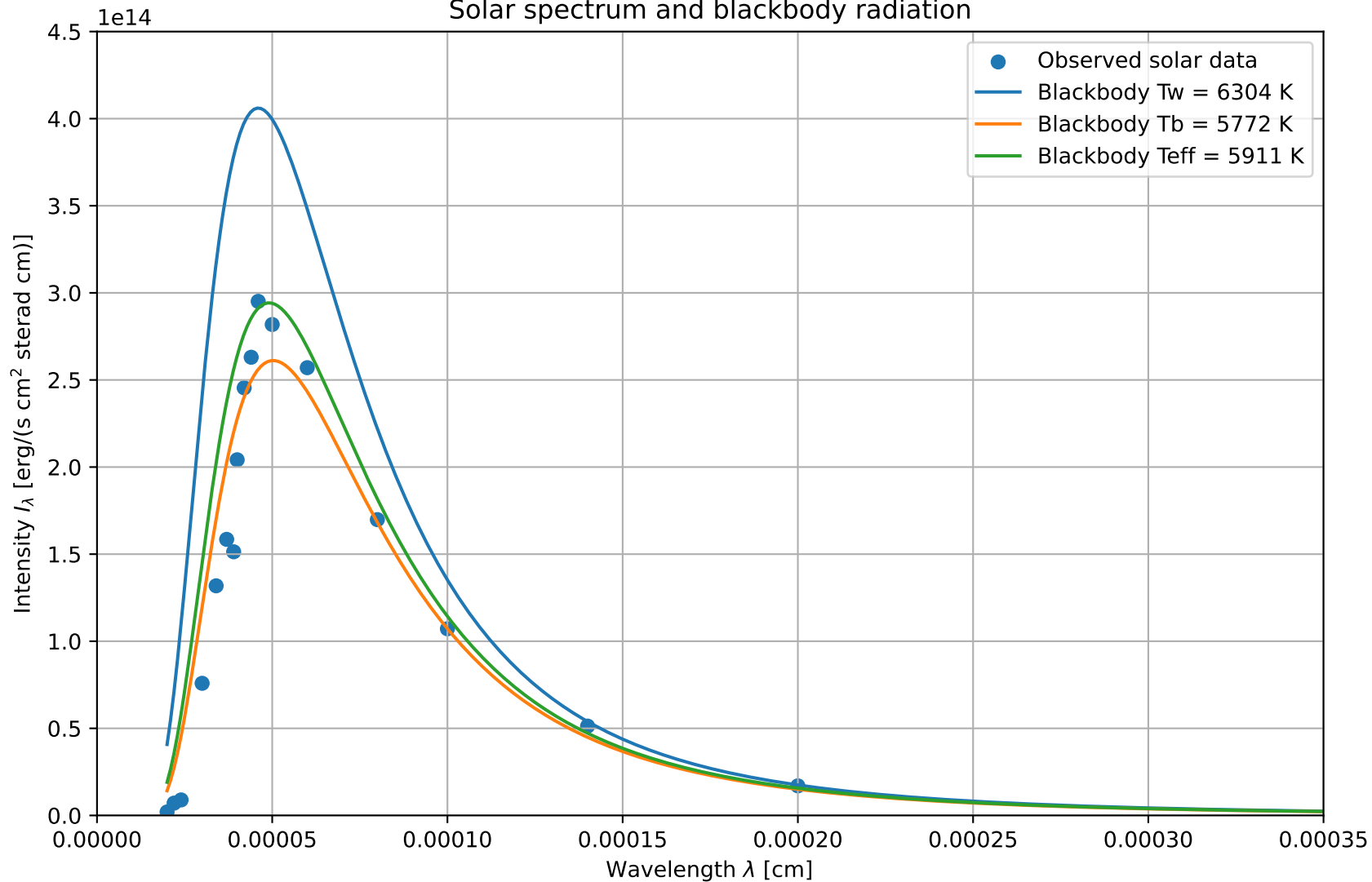
Solar spectrum and blackbody radiation
