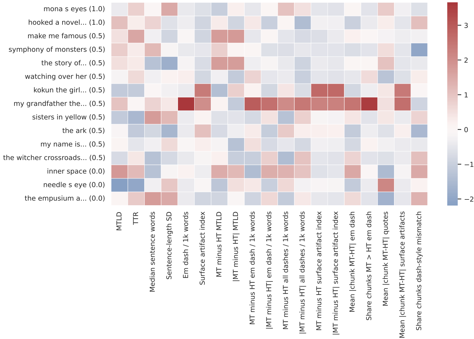
Primary feature z-scores by book, ordered by undetected rate
