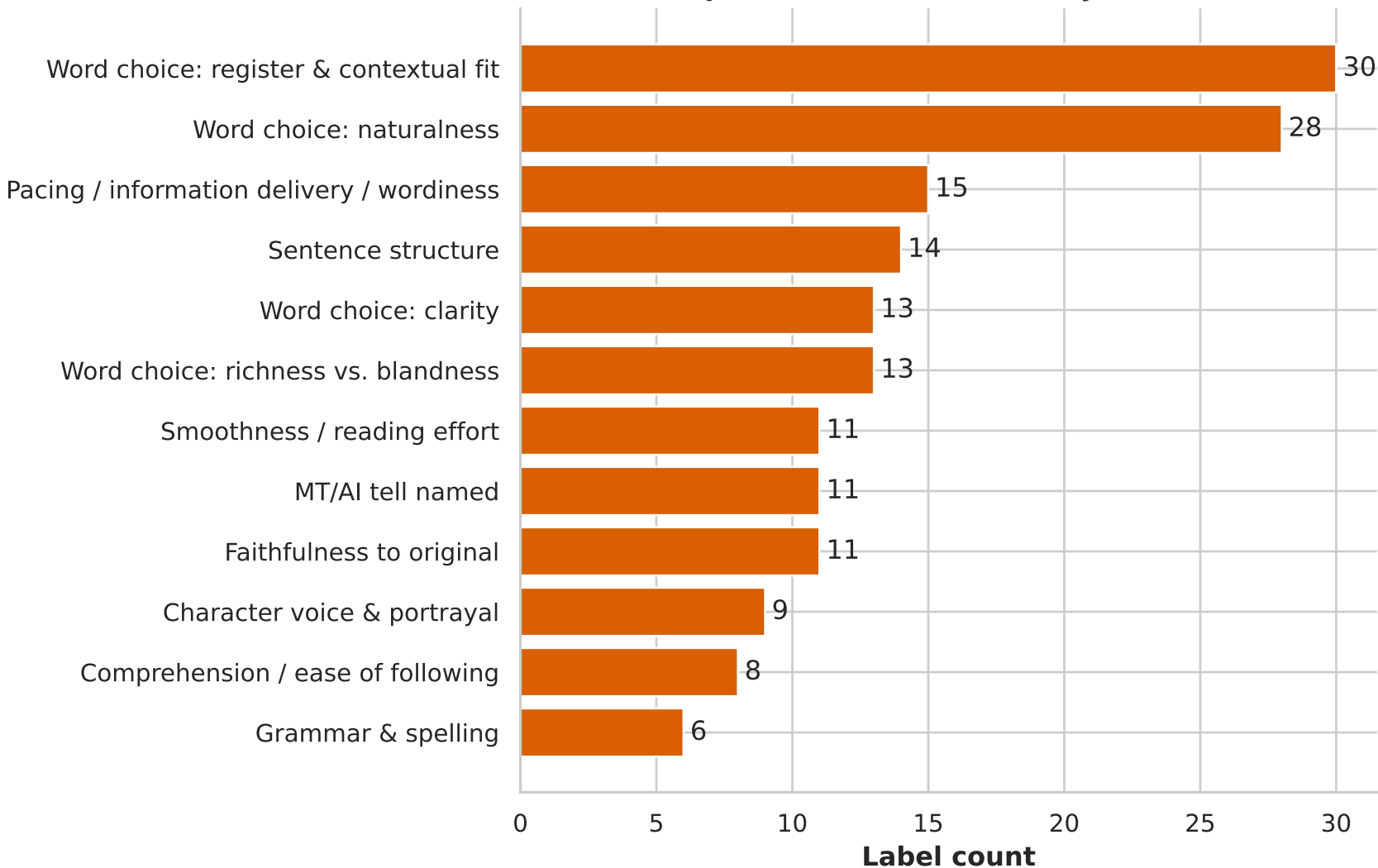
Top chunk NEG labels for rejected HT
