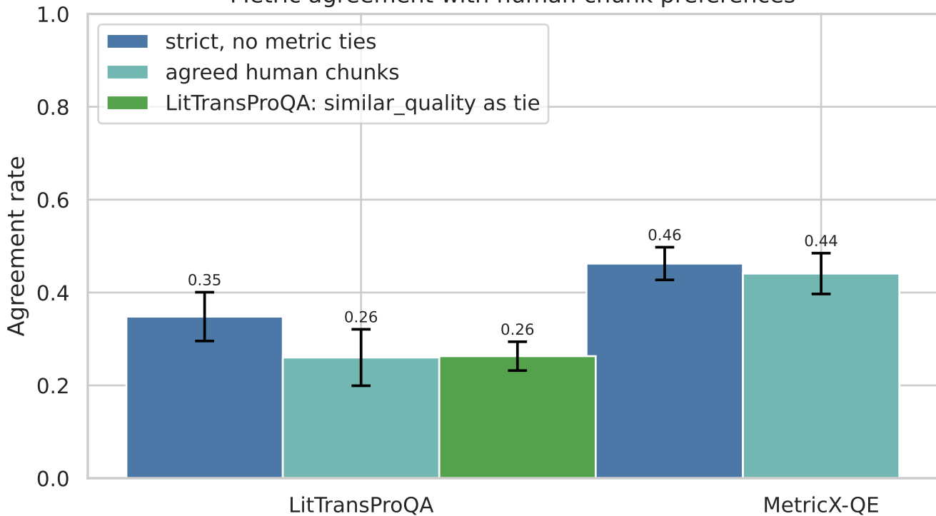
Metric agreement with human chunk preferences
