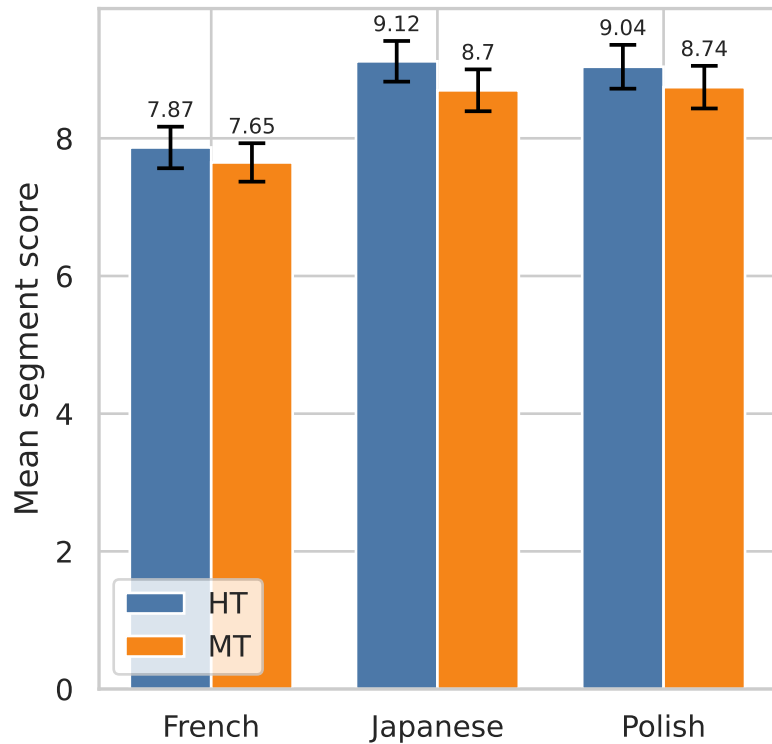
MetricX-QE
