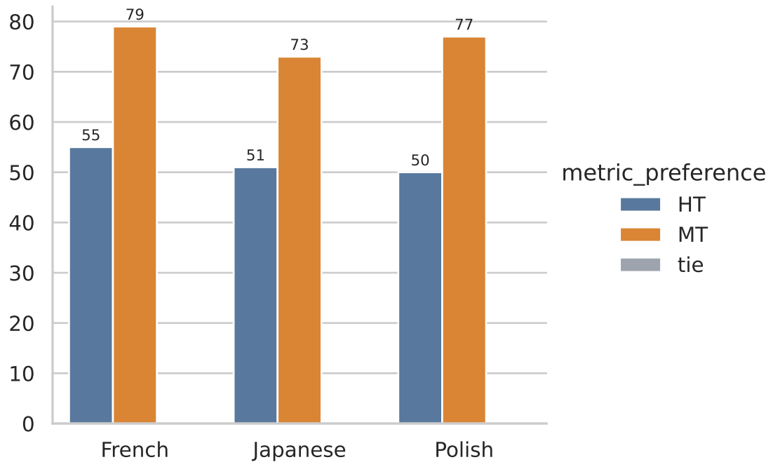
MetricX-QE
