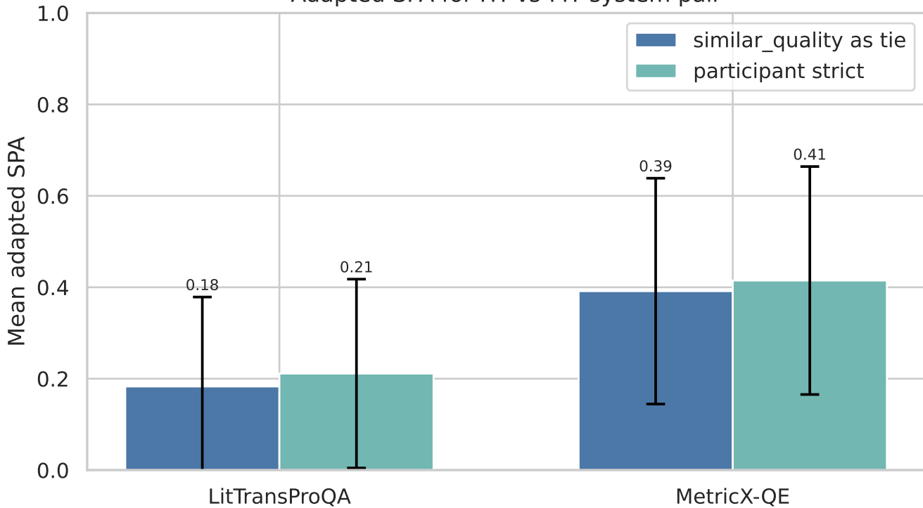
Adapted SPA for HT-vs-MT system pair
