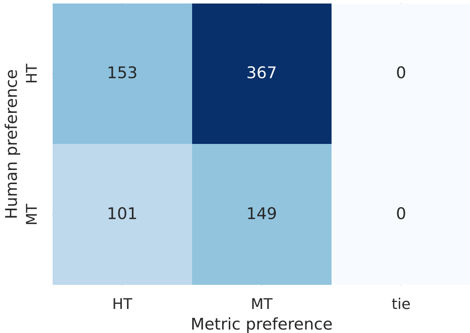
Human vs MetricX-QE (paragraph mean) preference
