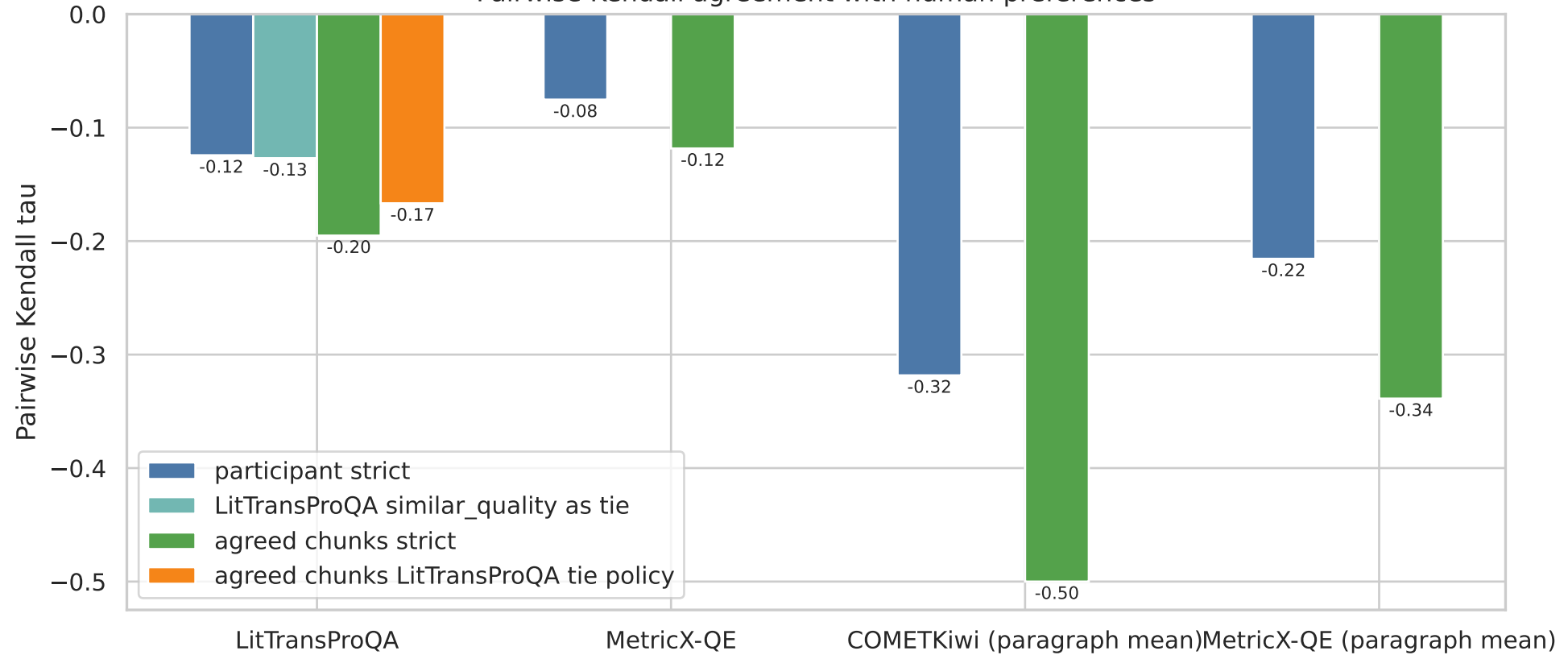
Pairwise Kendall agreement with human preferences
