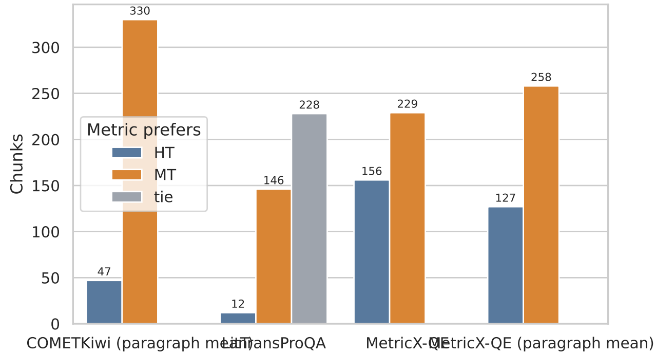
Metric preference counts
