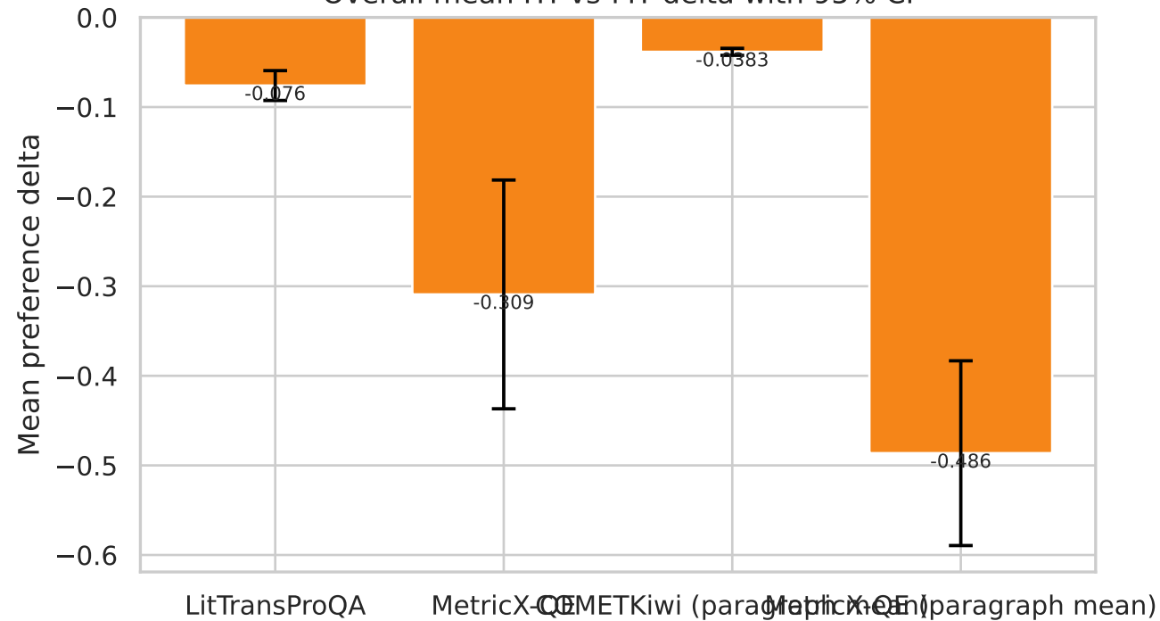
Overall mean HT-vs-MT delta with 95% CI
