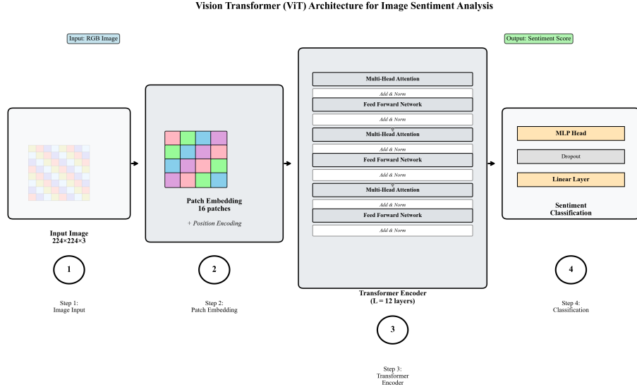
FIGURE 1. DETAILED ViT ARCHITECTURE
