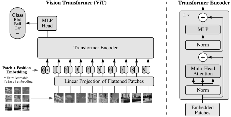
FIGURE 1. VISION TRANSFORMER ARCHITECTURE. THE MODEL PARTITIONS AN INPUT IMAGE INTO FIXED-SIZE PATCHES, LINEARLY PROJECTS THEM INTO TOKEN EMBEDDINGS, PREPENDS A LEARNABLE [\text{class}] TOKEN, ADDS POSITIONAL EMBEDDINGS, AND FEEDS THE RESULTING SEQUENCE THROUGH A STACK OF STANDARD TRANSFORMER ENCODER BLOCKS (RIGHT PANEL). IMAGE SOURCE: DOSOVITSKIY ET AL. (2020), FIGURE 1, REPRODUCED UNDER ARXIV NON-EXCLUSIVE ACADEMIC-USE LICENSE.
