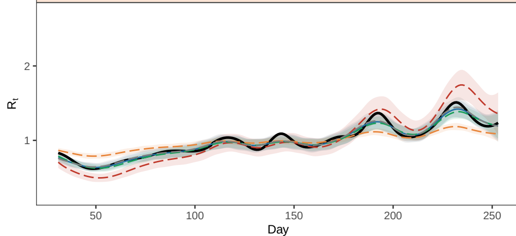
E. Estimated R_t over time (EpiLPS (MALA))
