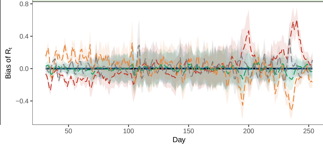
D. Time-varying bias (EpiLPS (MAP))
