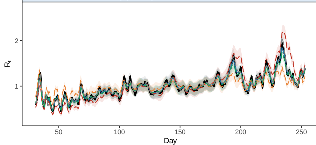
G. Estimated R_t over time (EpiFilter)
