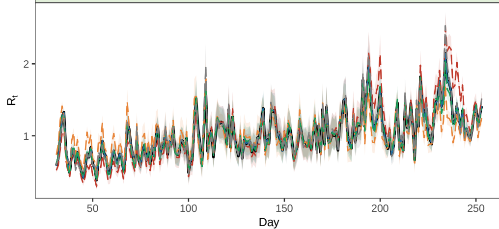
C. Estimated R_t over time (EpiLPS (MAP))
