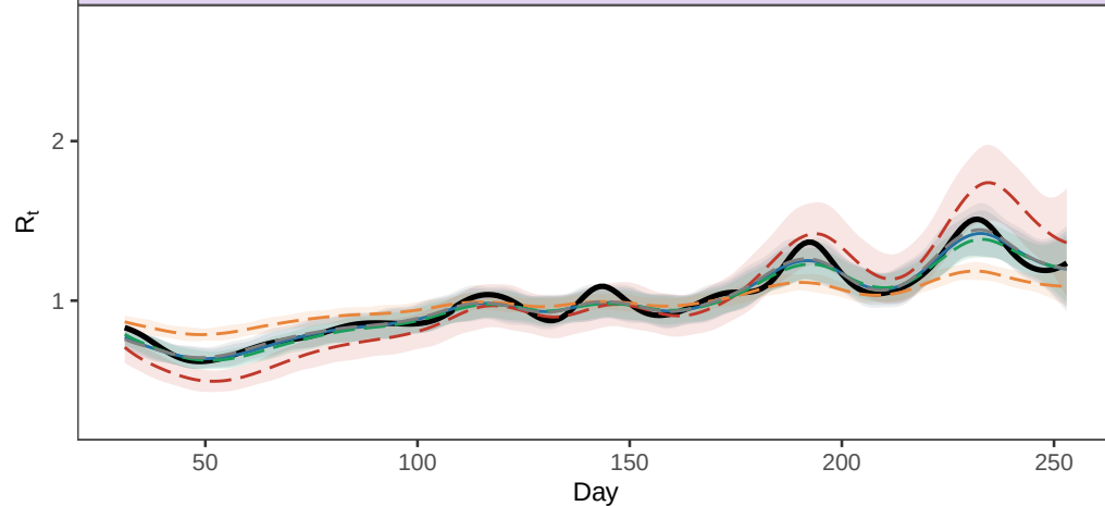
G. Estimated R_t over time (EpiFilter)
