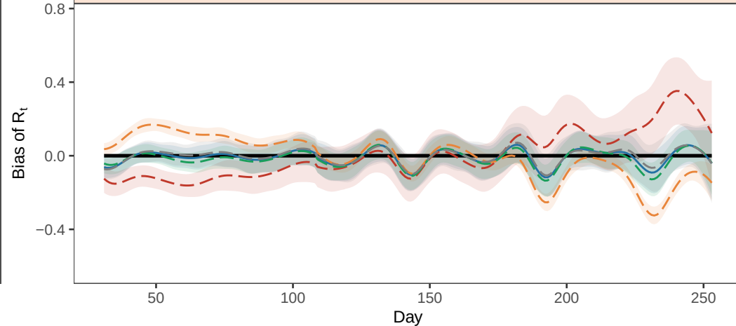
F. Time-varying bias (EpiLPS (MALA))
