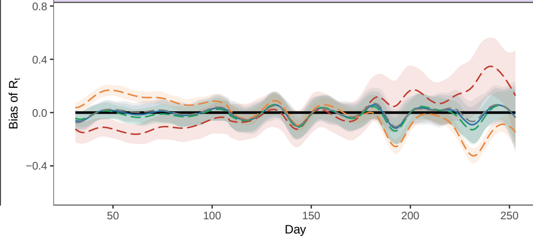
H. Time-varying bias (EpiFilter)
