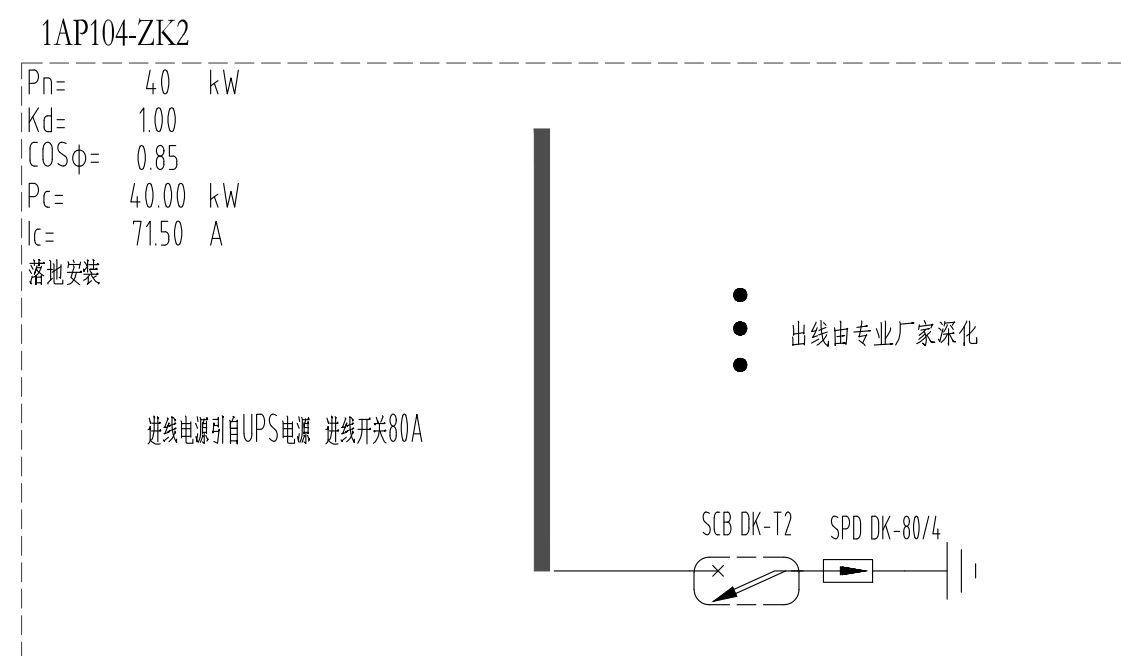
MPC总控机房配电箱2
