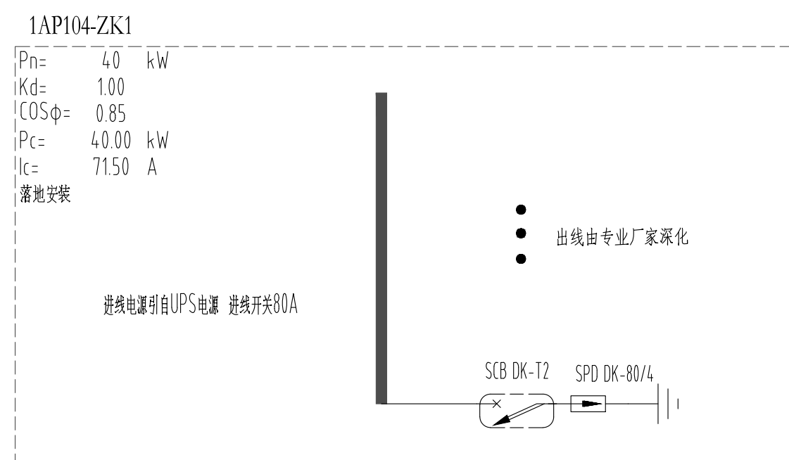
MPC总控机房配电箱1
