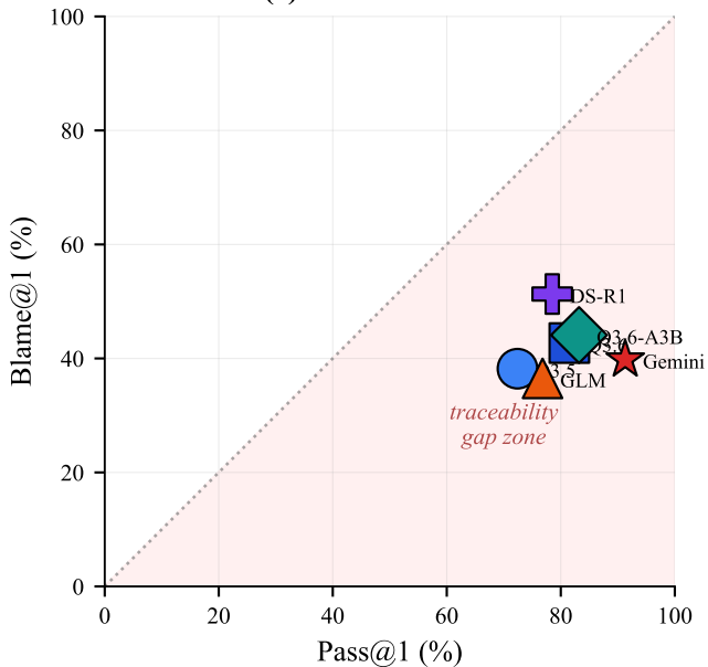
(a) TraceBench-Full
