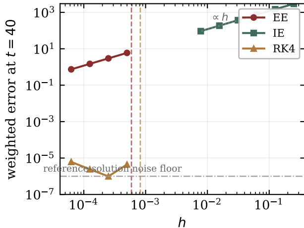
Stiff problem: convergence and stability cut-offs
