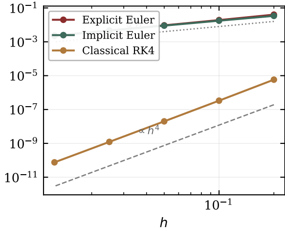
Order verification (Prothero-Robinson, \lambda = -1 )
