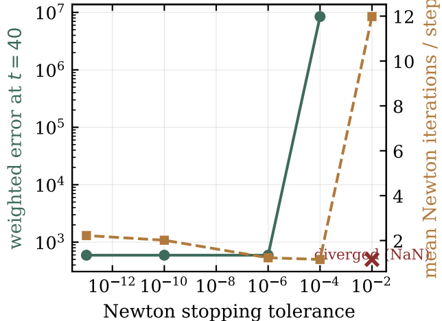
Inexact Newton: accuracy vs. cost
