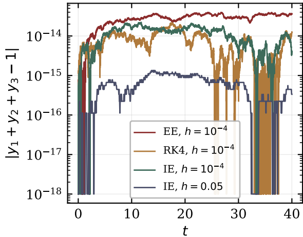
Invariant defect stays at round-off
