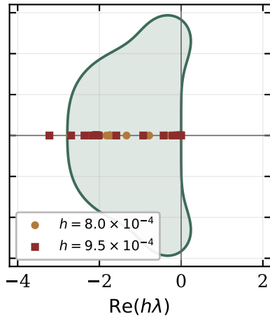
Classical RK4
