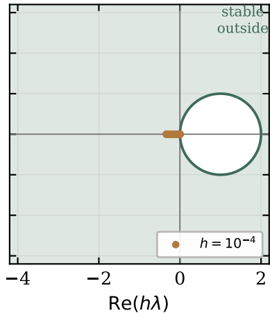
Implicit Euler
