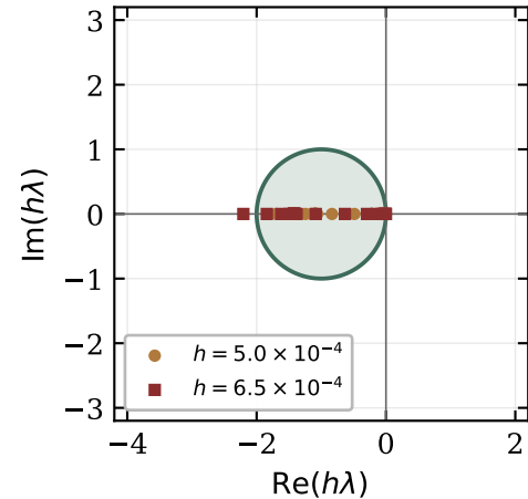
Explicit Euler
