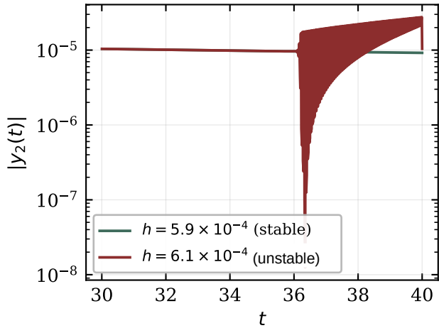
Explicit Euler: late-time view
