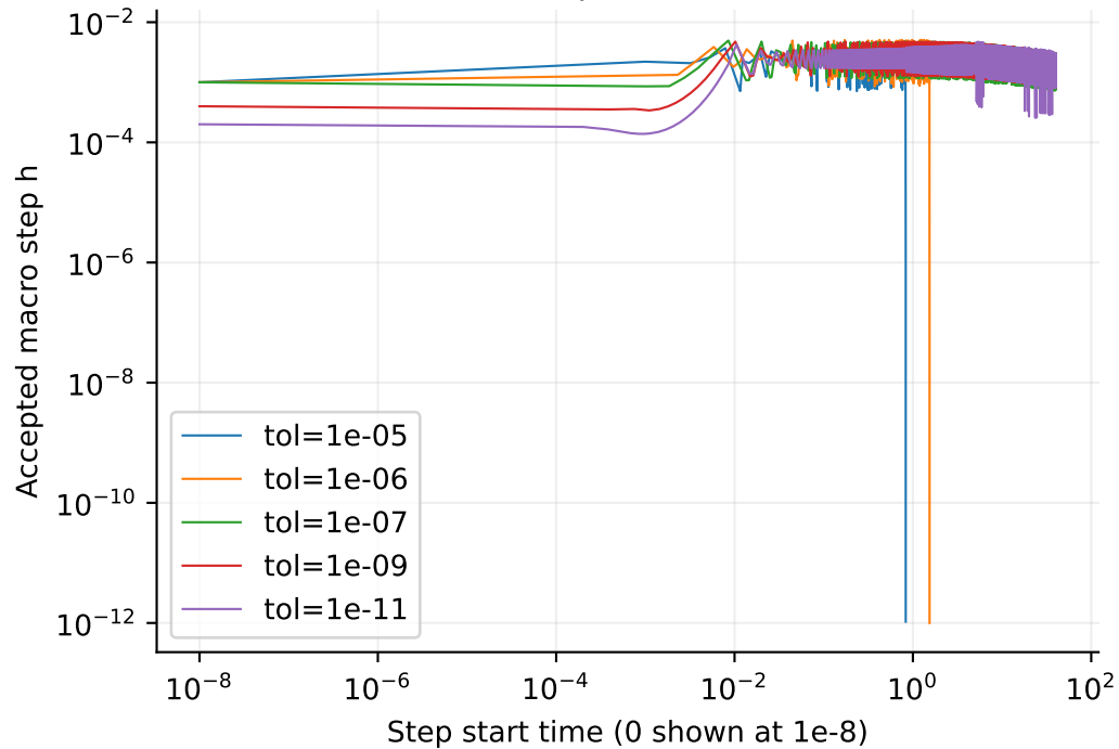
Adaptive RK4
