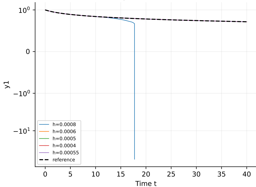
Slow species and failure
