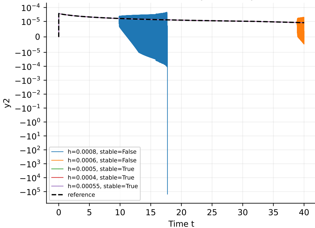
EE near the stability boundary
