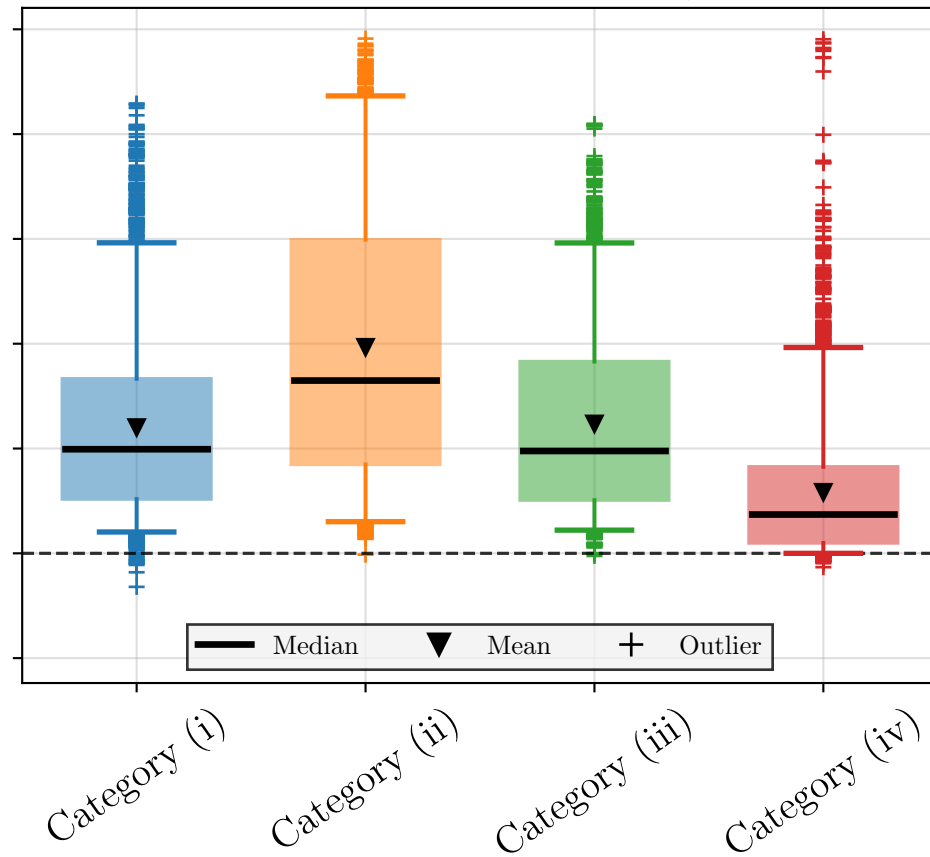
Discounted-pipeline policy
