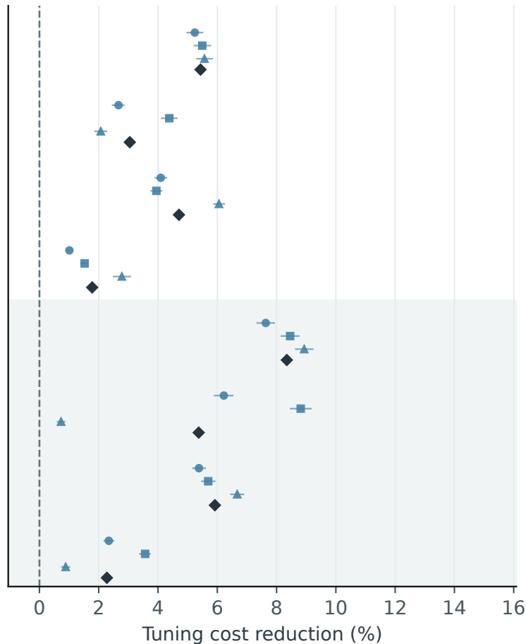
Best of 8
