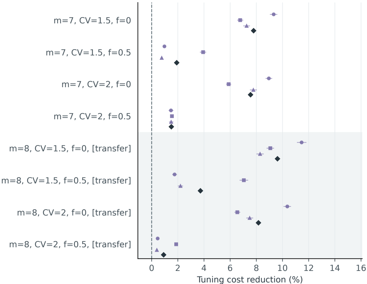
One query
