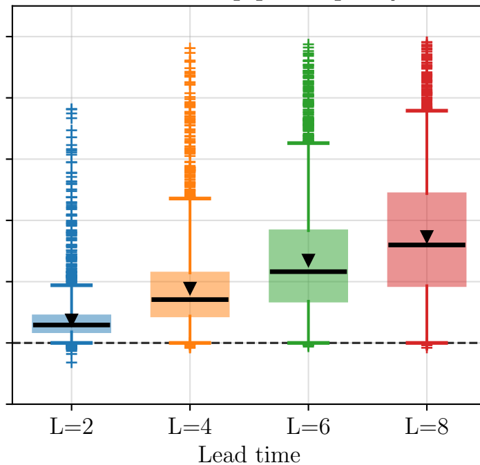
Discounted-pipeline policy
