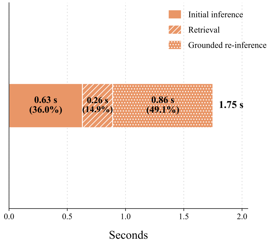
(b) Runtime composition of retrieval-augmented grounding
