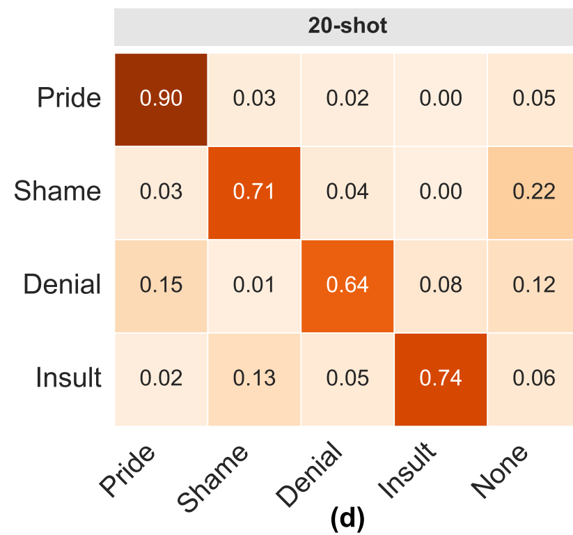
Predicted label
